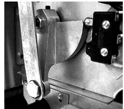
Left bell crank and cam with basket lift link shown in down position. Note microswitch in upper right corner.
