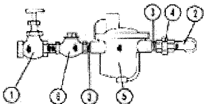
Condensate Outlet Piping
